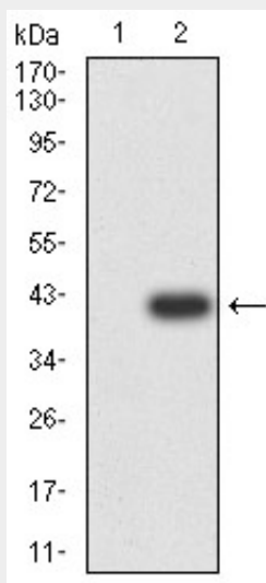
Figure 3: Western blot analysis using CD3G mAb against HEK293 (1) and CD3G (AA: extra 23-116)-hlgGFc transfected HEK293 (2) cell lysate.
