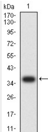
Figure 2: Western blot analysis using CD3G mAb against human CD3G (AA: extra 23-116) recombinant protein. (Expected MW is 36.6 kDa)
